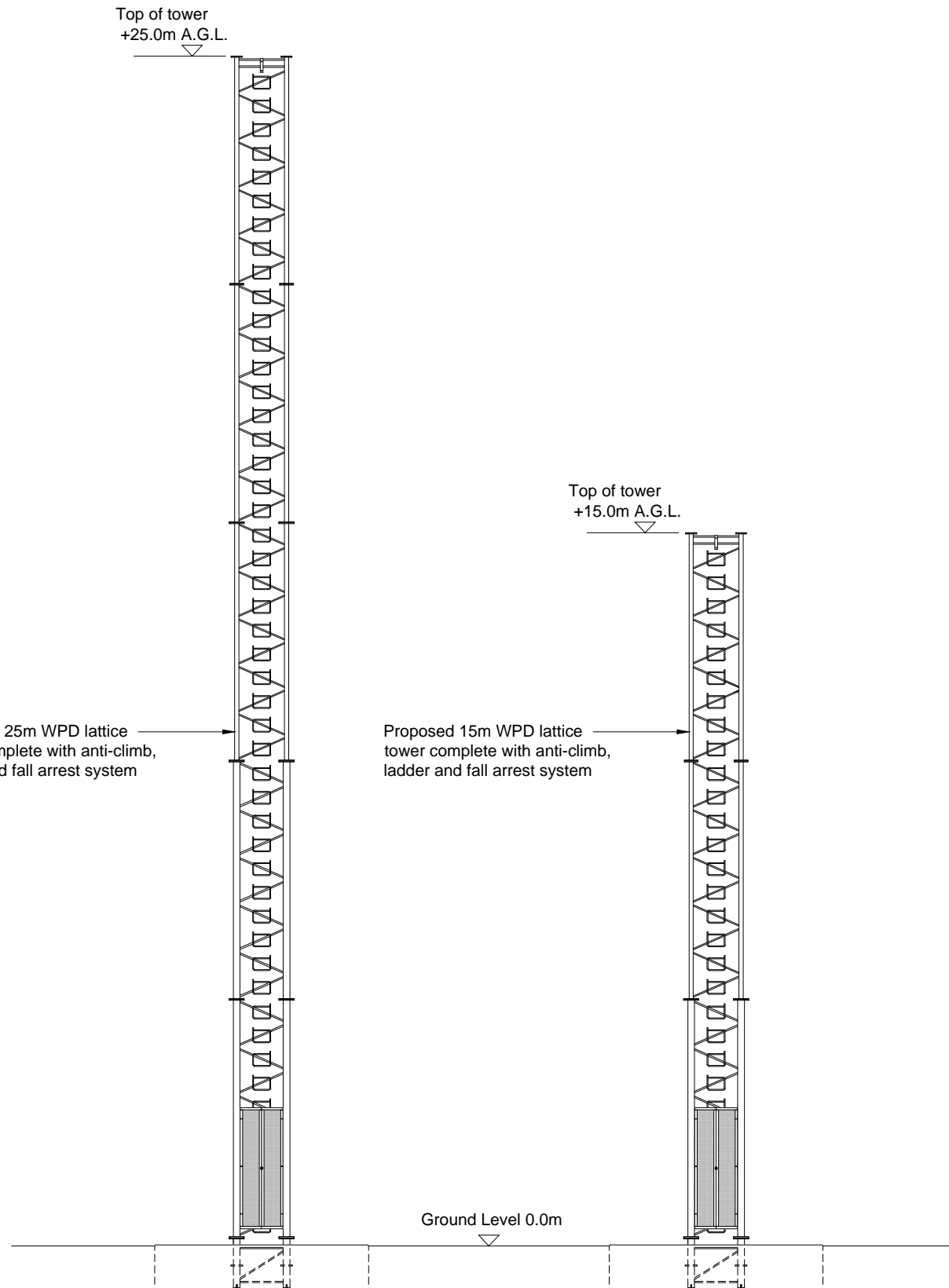
TYPICAL TOWER ELEVATION
